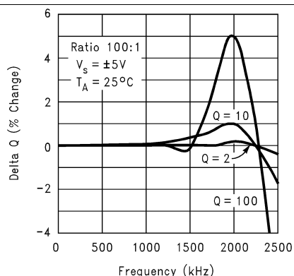
Figure 19. Q Deviation vs Clock Frequency
